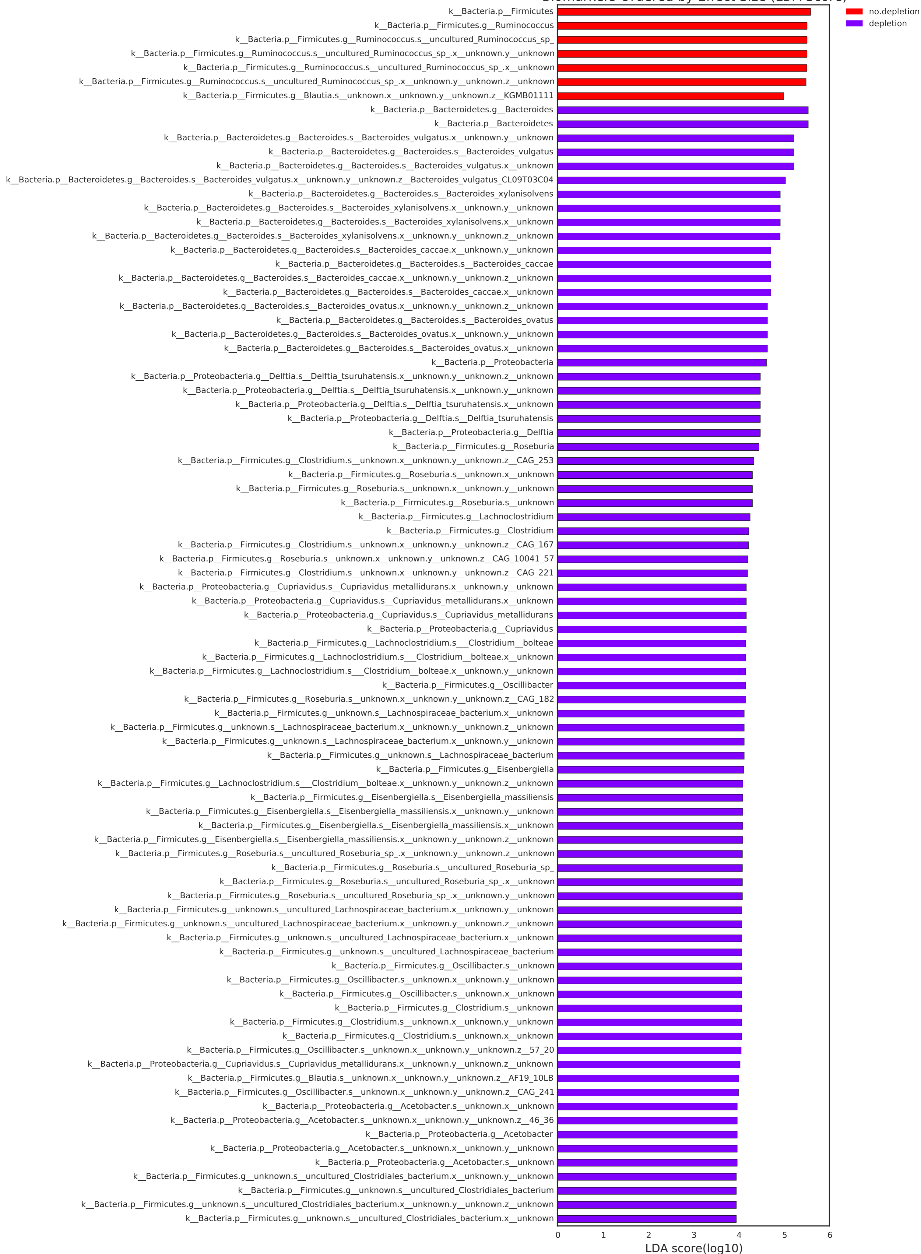
Biomarkers Ordered by Effect Size (LDA Score)
