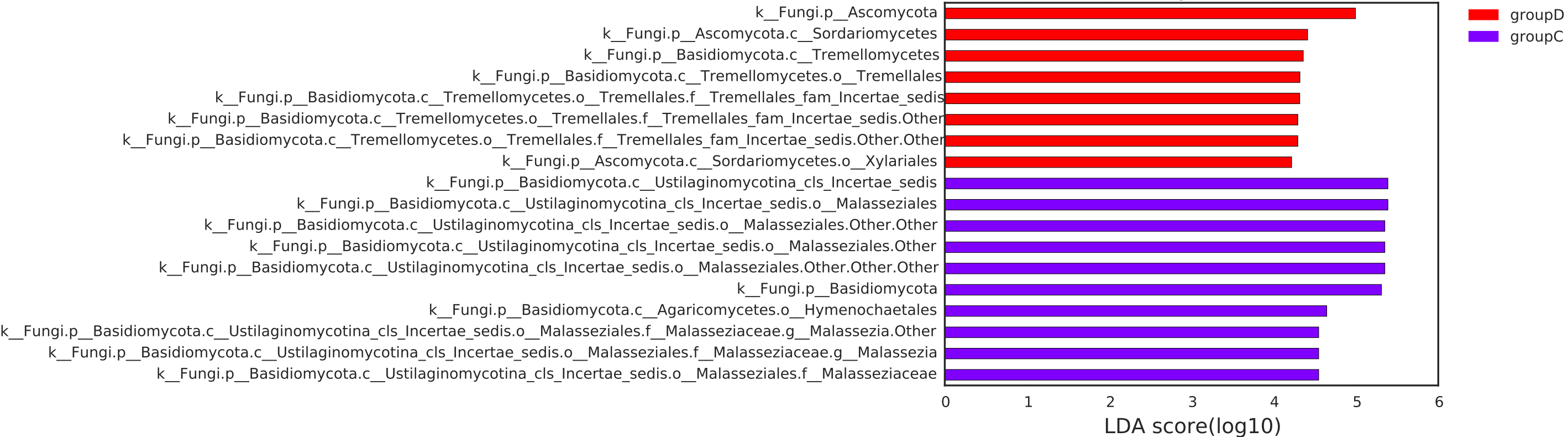
Biomarkers Ordered by Effect Size (LDA Score)
